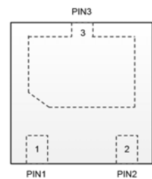
PIN Configuration
