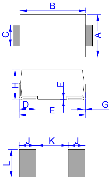
DO-214AA (SMB)
